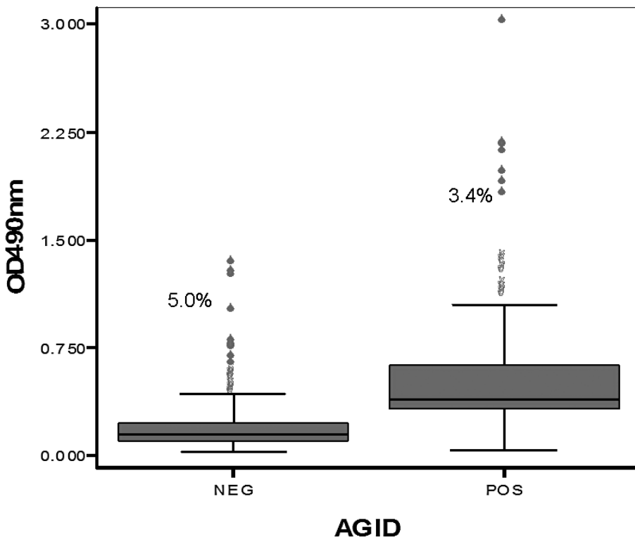
FIGURE 2. The interactive box file plot using the SPSS program. The scatterplot indicate the relationship of the AGID positive and negative results with the optical density reading at 490 nm for the ELISA assay.
