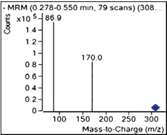
Figure 1. Product ion scan of SA, m/z 307.99, showing the most intense fragment ions at m/z 86.9 and 170
